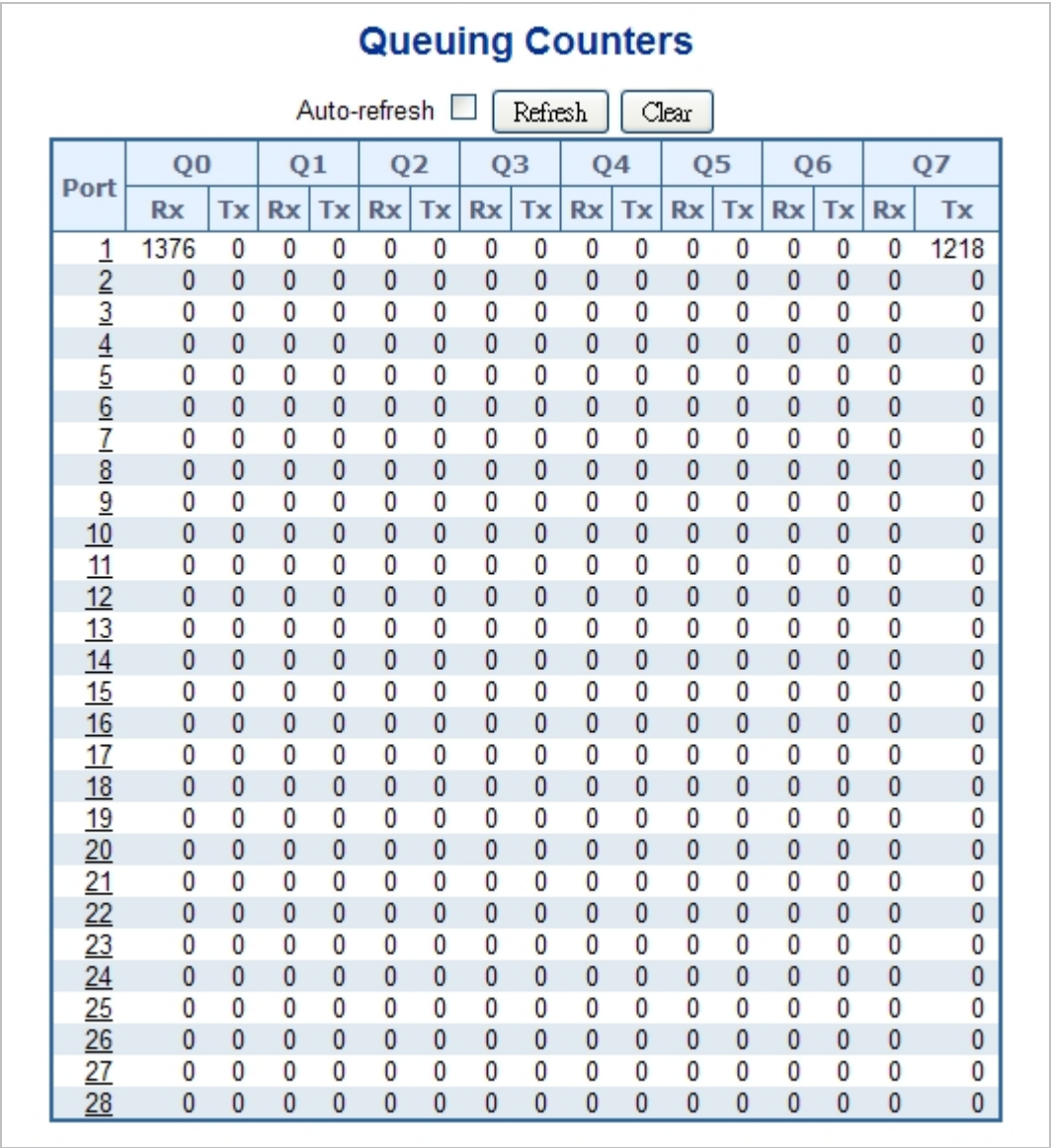
Figure 4-9-17: Queuing Counters Page Screenshot
