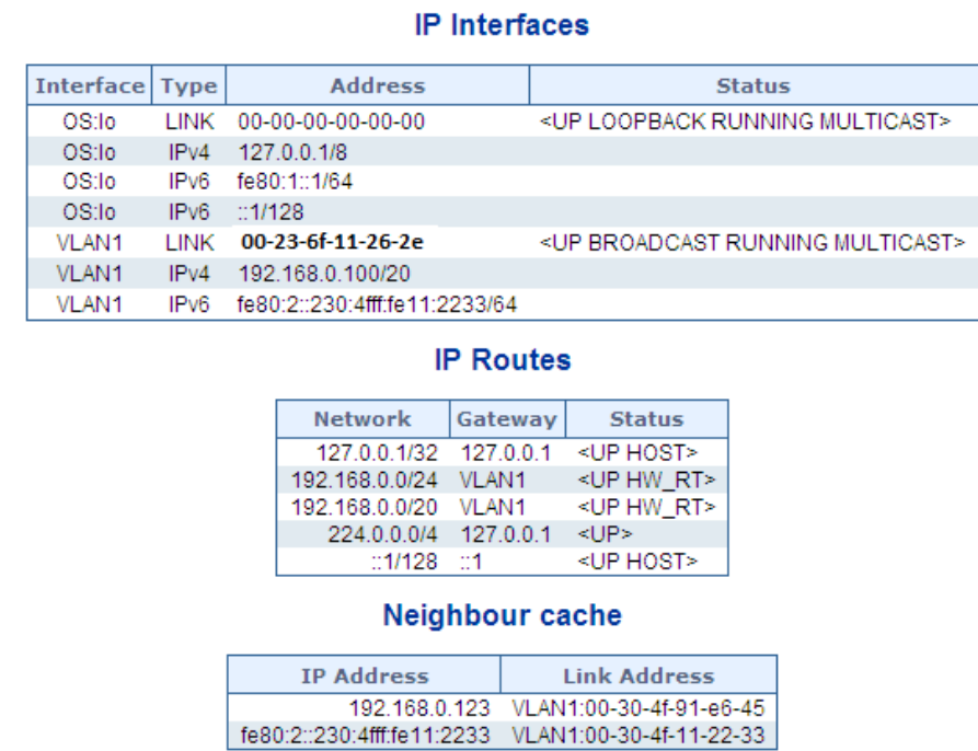
Figure 4-2-3: IPv6 Configuration Page Screenshot
