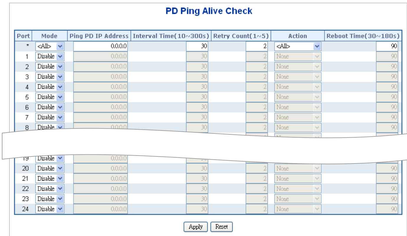
Figure 4-16-9: PD Alive Check Configuration Screenshot
