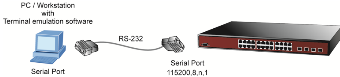
Figure 3-1-1: Console Management
