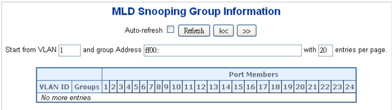
Figure 4-8-17: MLD Snooping Groups Information Page Screenshot
