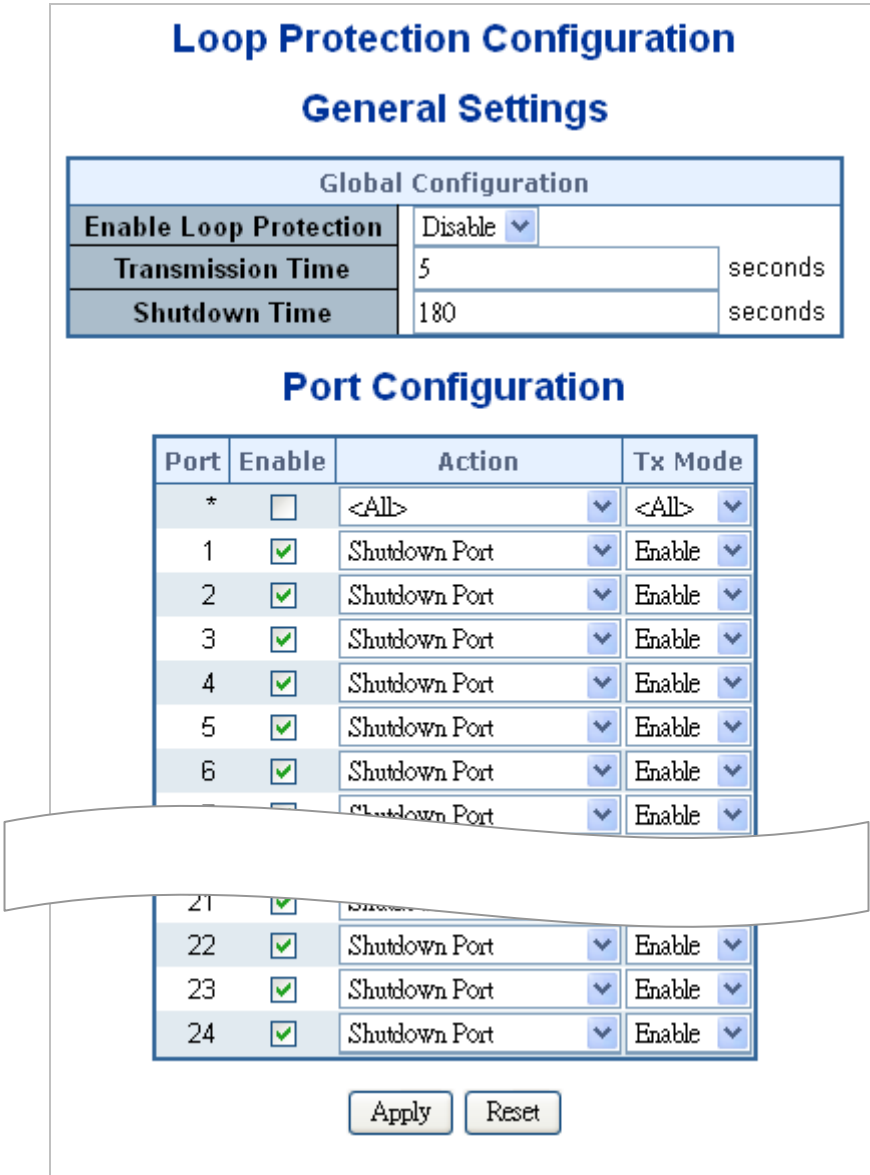
Figure 4-17-1: Loop Protection Configuration Page Screenshot
