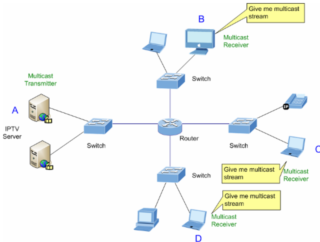
Figure 4-8-1: Multicast Service
