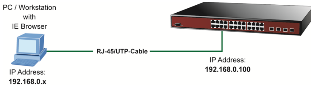
Figure 3-1-3: Web Management
