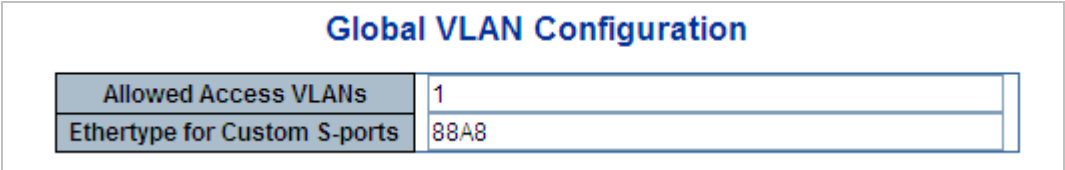
Figure 4-6-1 : Global VLAN Configuration Screenshot
