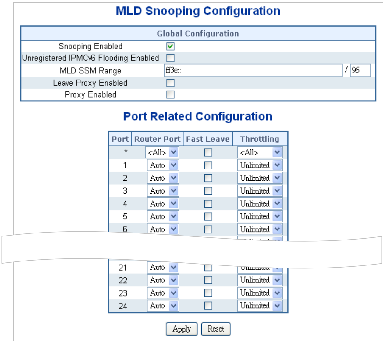
Figure 4-8-13: MLD Snooping Configuration Page Screenshot
