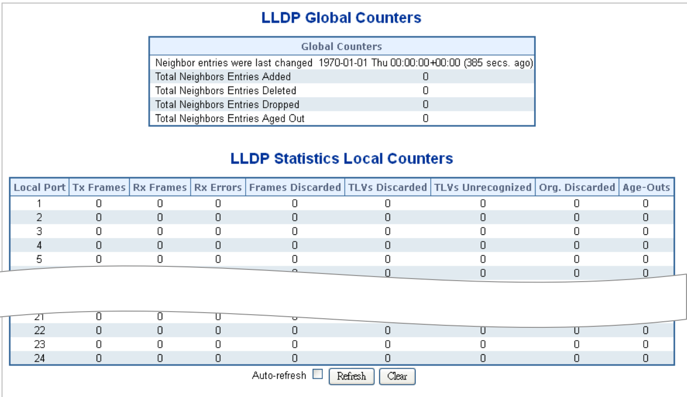
Figure 4-14-5: LLDP Statistics Page Screenshot
