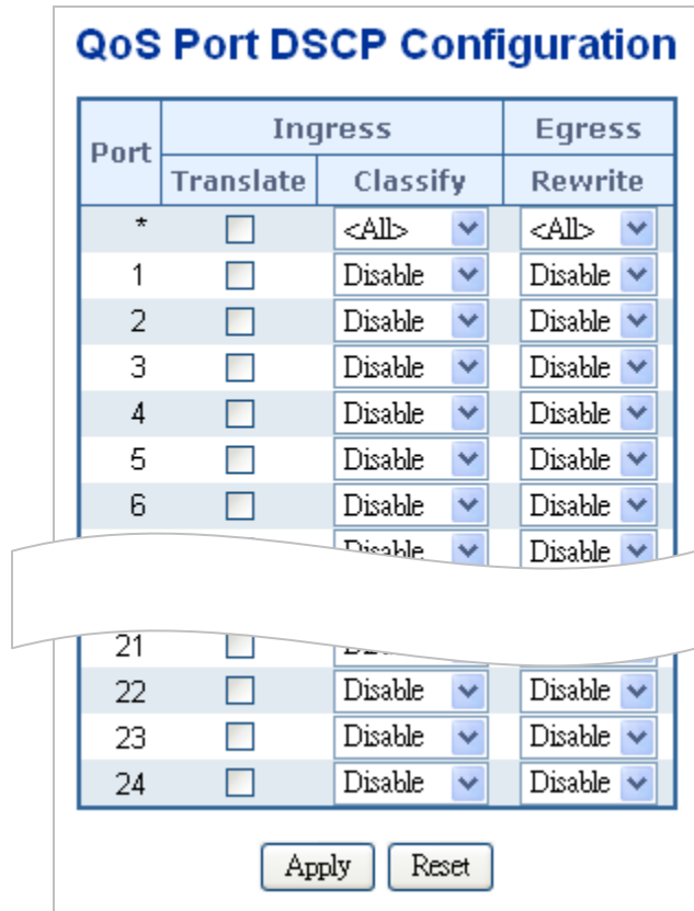
Figure 4-9-8: QoS Port DSCP Configuration Page Screenshot
