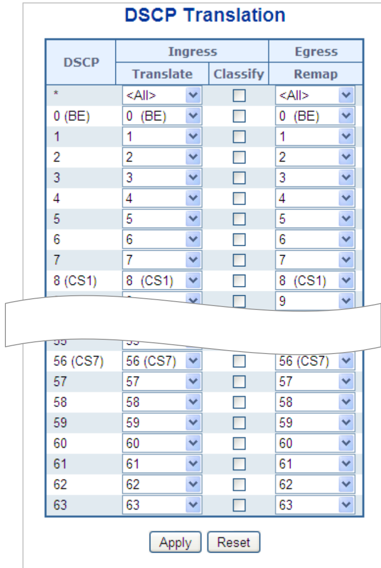
Figure 4-9-10: DSCP Translation Page Screenshot
