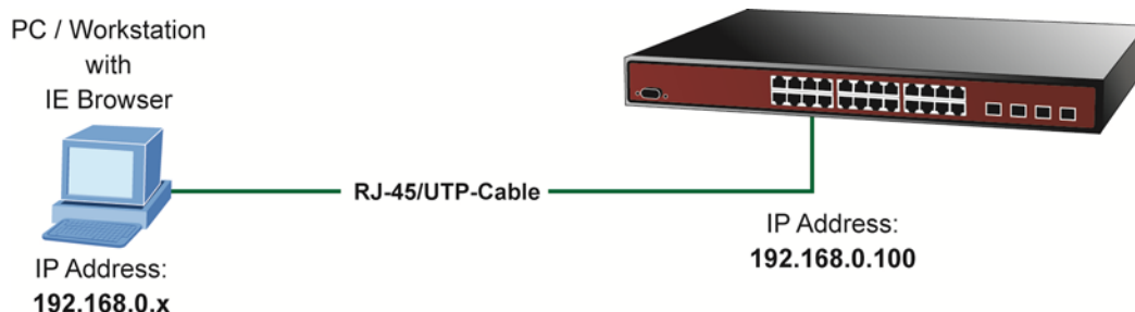
Figure 4-1-1: Web Management
