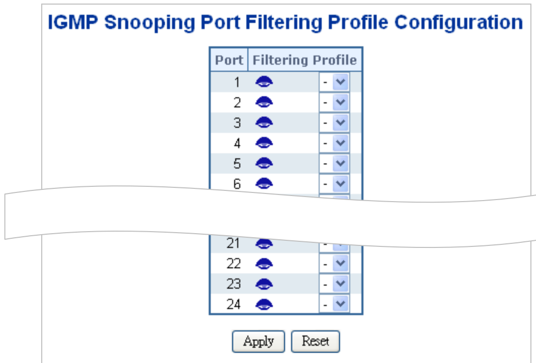
Figure 4-8-9: IGMP Snooping Port Filtering Profile Configuration Page Screenshot
