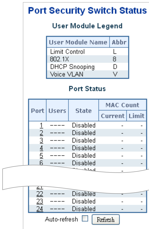
Figure 4-12-6: Port Security Status Screen Page Screenshot
