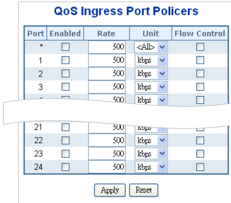
Figure 4-9-1: QoS Ingress Port Policers Page Screenshot
