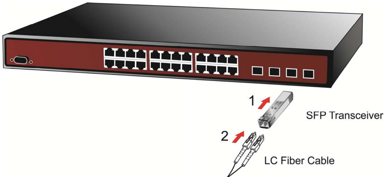
Figure 2-2-4: Plug-in the SFP Transceiver
