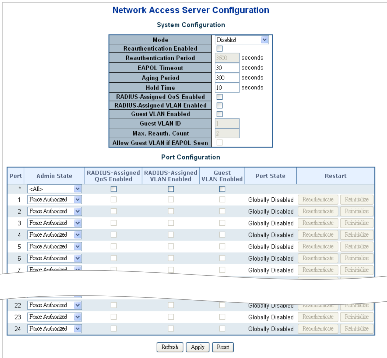
Figure 4-11-4: Network Access Server Configuration Page Screenshot
