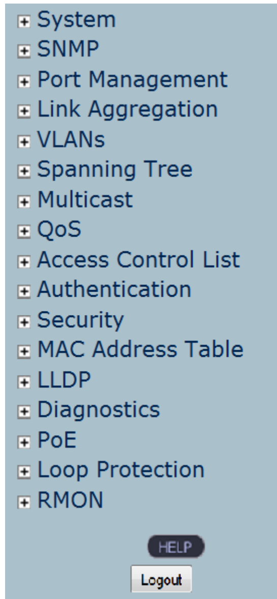
Figure 4-1-5: Managed Switch Main Functions Menu
