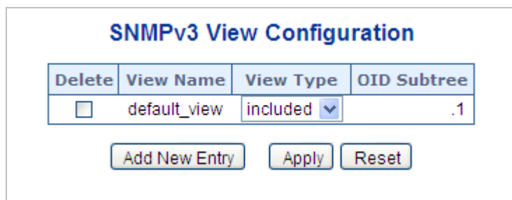
Figure 4-3-7: SNMPv3 Views Configuration Page Screenshot
