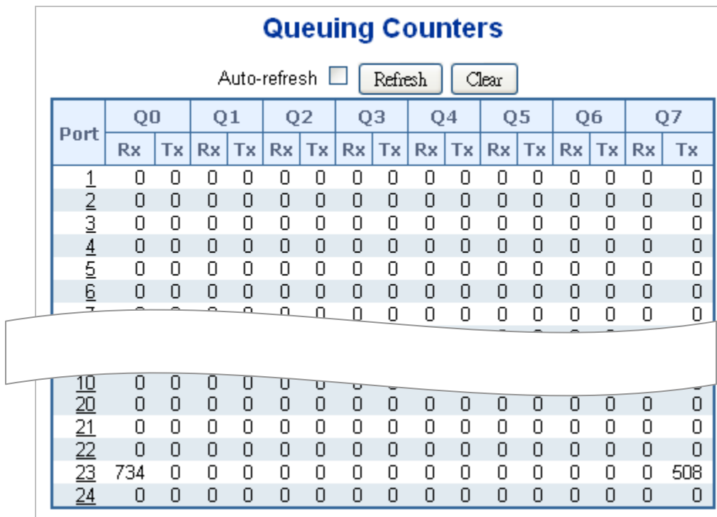
Figure 4-9-17: Queuing Counters Page Screenshot
