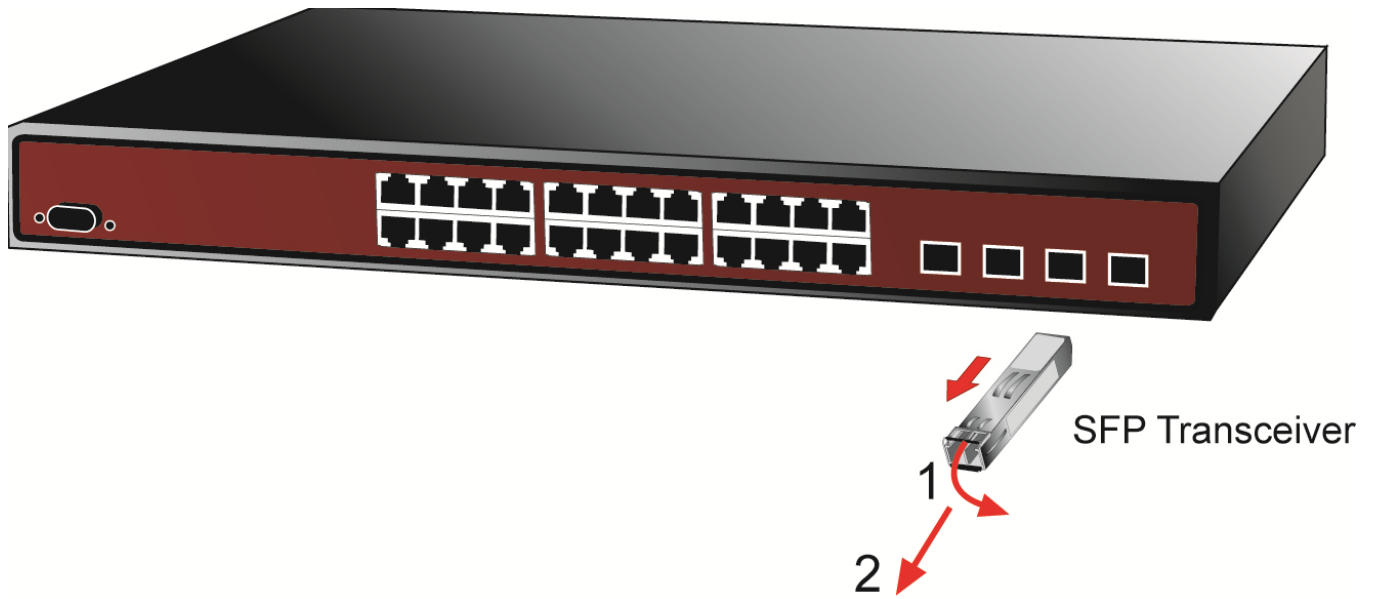
Figure 2-2-5: How to Pull Out the SFP/SFP+ Transceiver
