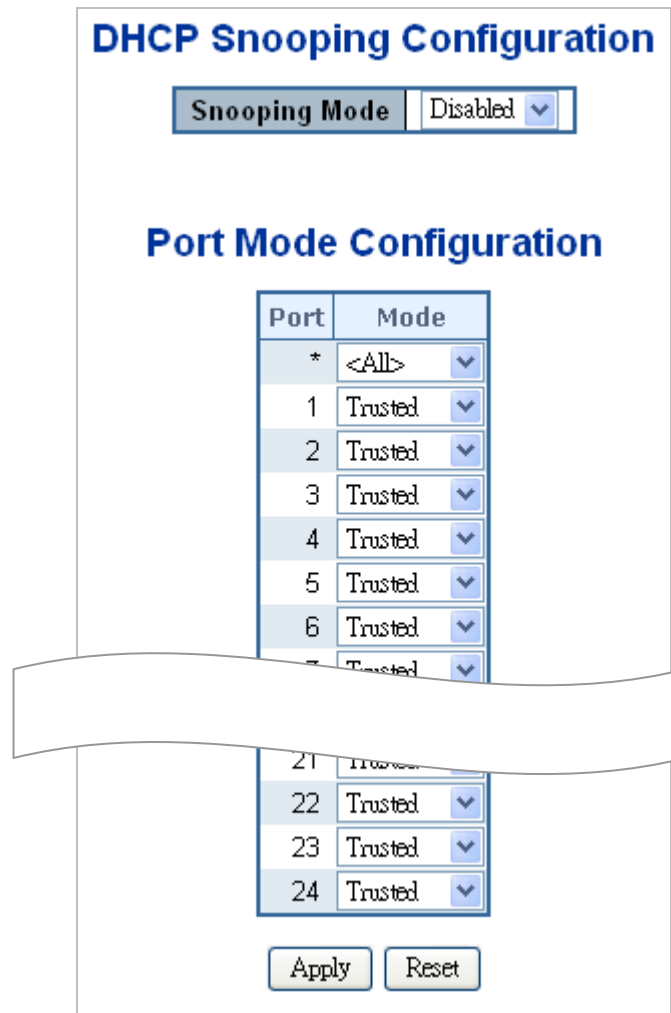
Figure 4-12-8: DHCP Snooping Configuration Screen Page Screenshot
