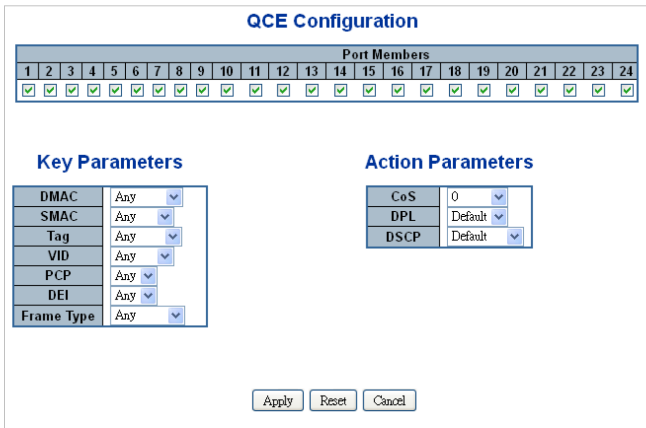
Figure 4-9-13: QCE Configuration Page Screenshot
