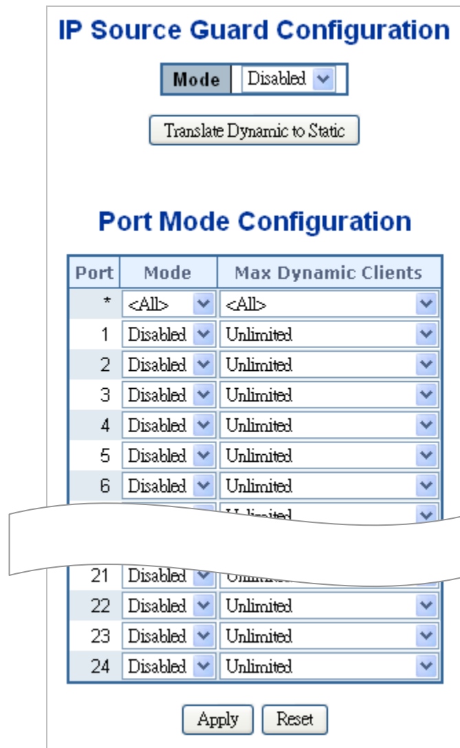
Figure 4-12-10: IP Source Guard Configuration Screen Page Screenshot
