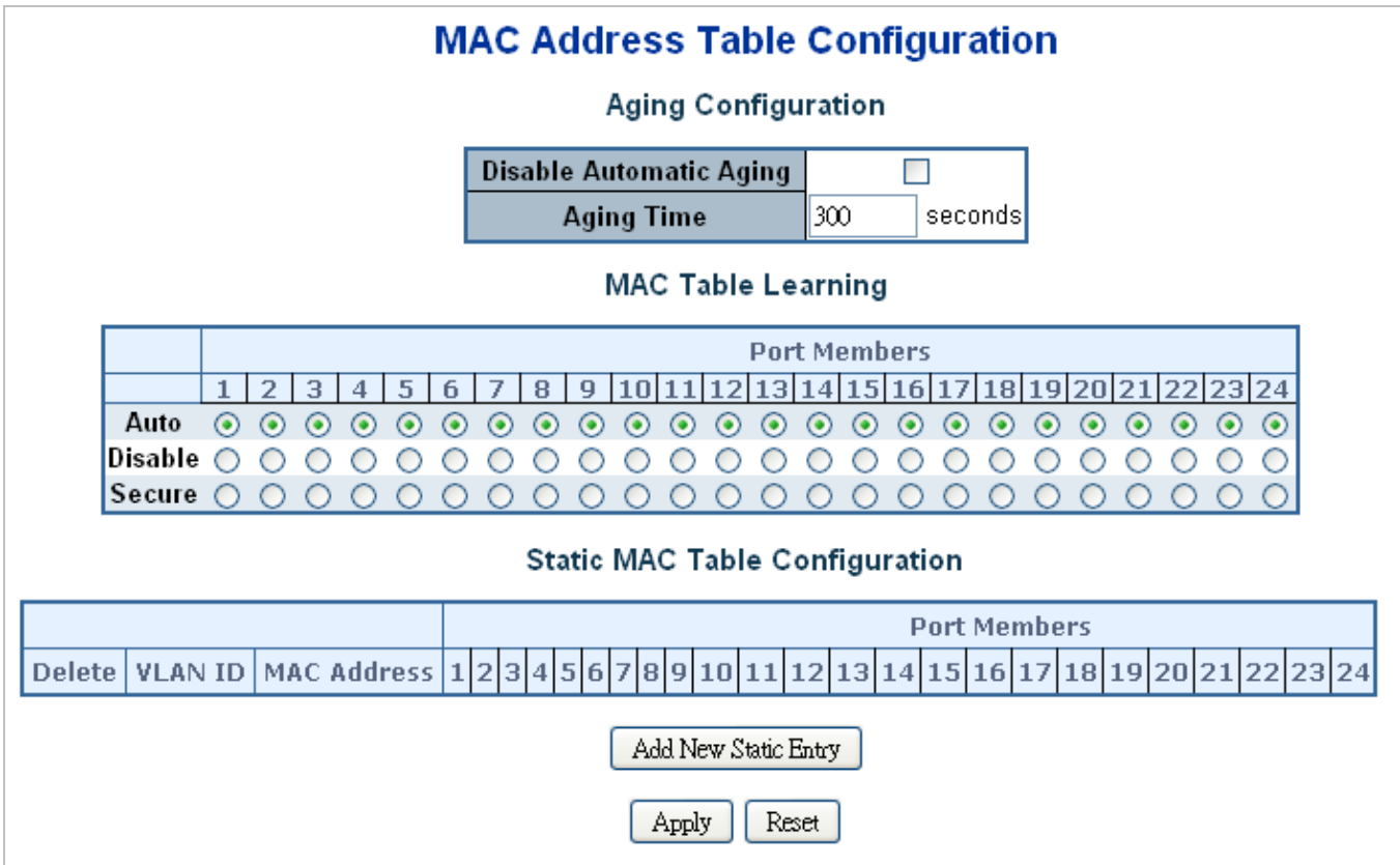
ure 4-13-1: MAC Address Table Configuration Page Screenshot
