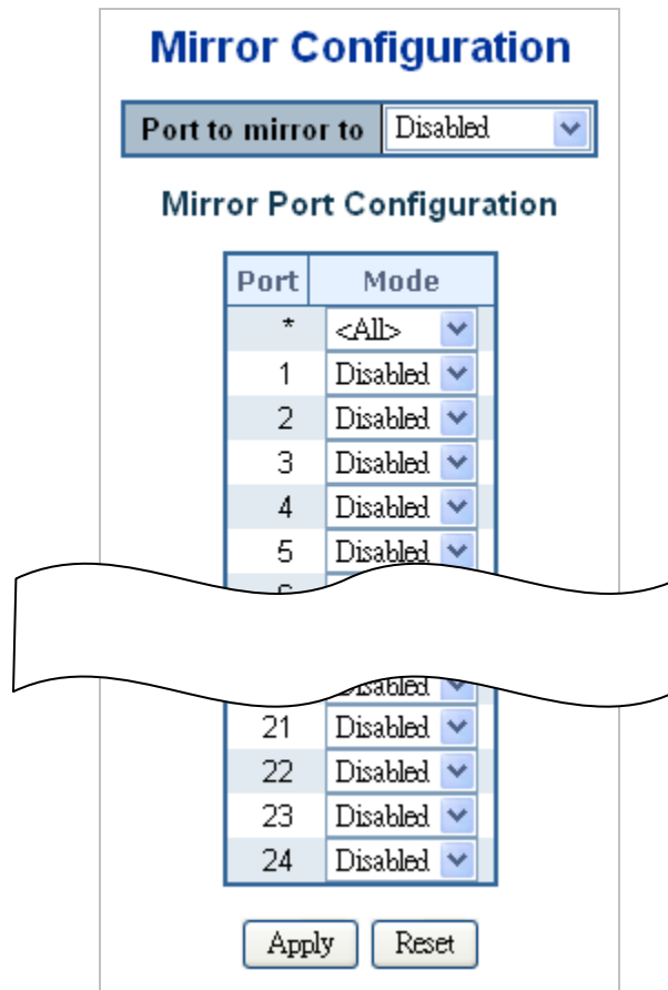
Figure 4-4-8: Mirror Configuration Page Screenshot
