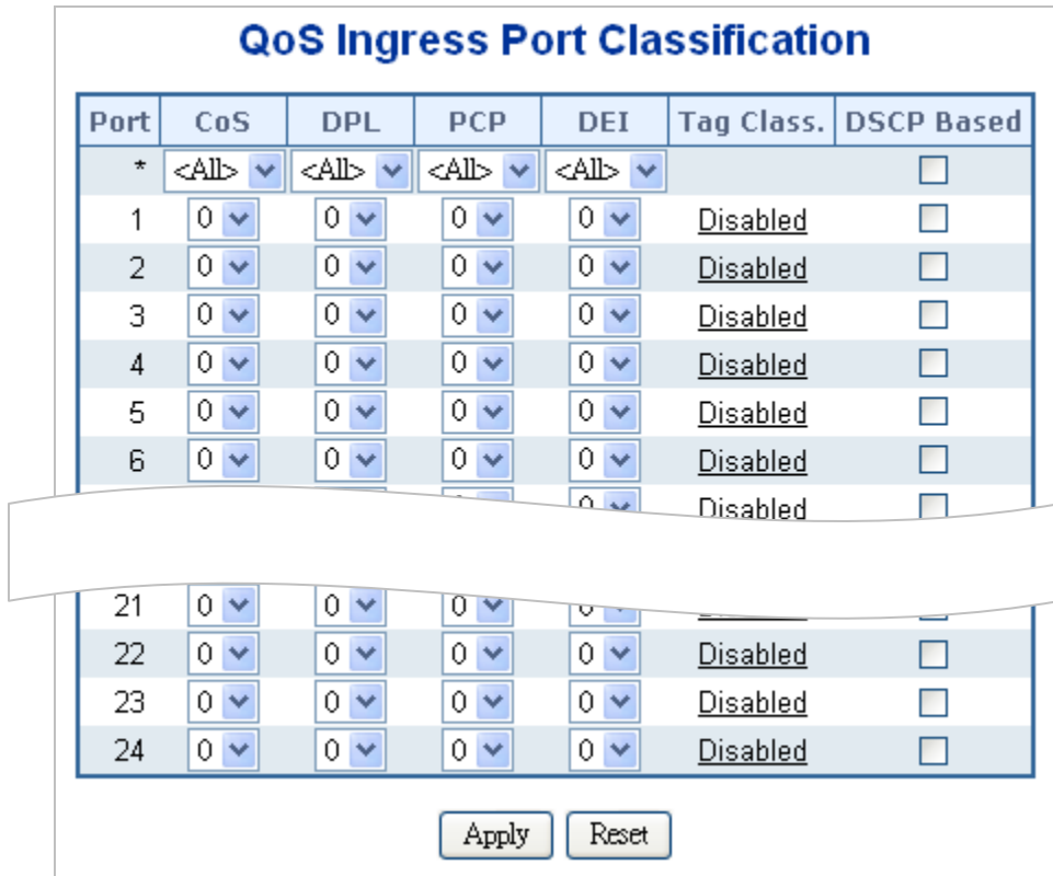
Figure 4-9-2 : QoS Ingress Port Classification Page Screenshot
