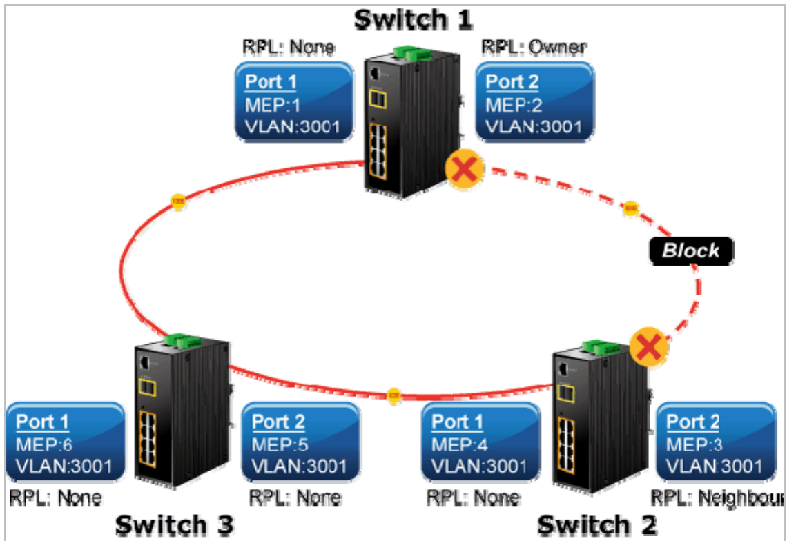
Figure 4-19-6: Ring Example Diagram
