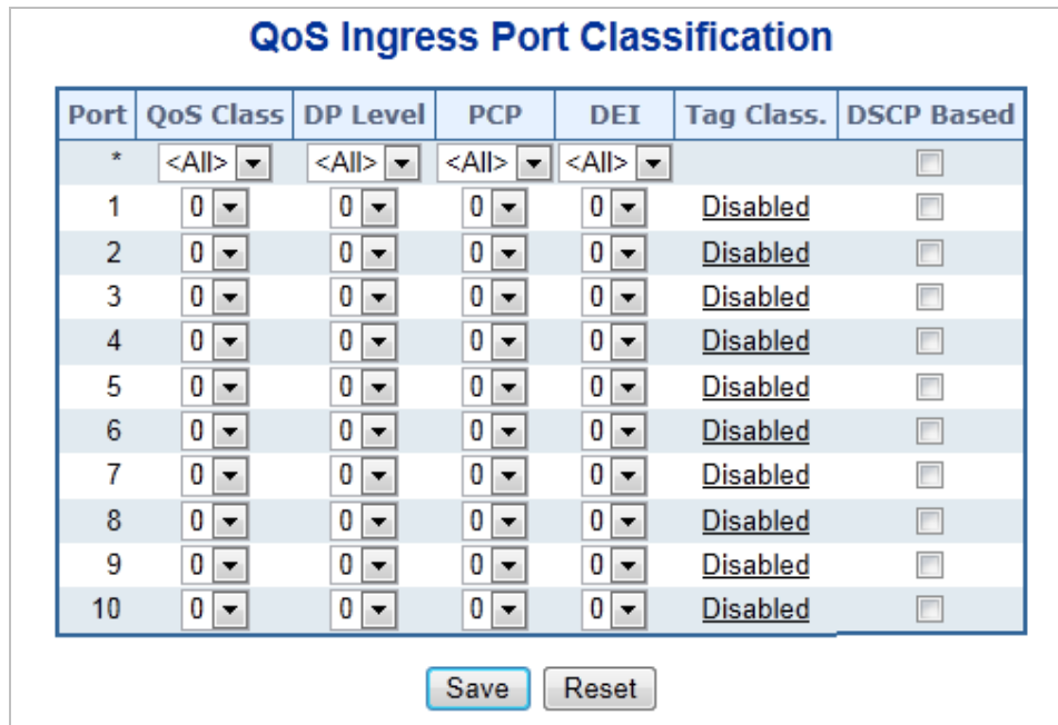
Figure 4-9-4 : QoS Ingres Port Classification Page Screenshot
