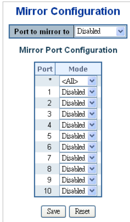
Figure 4-4-6: Mirror Configuration Page Screenshot
