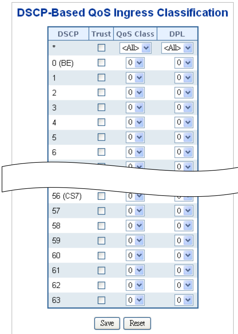
Figure 4-9-10: DSCP-Based QoS Ingress Classification Page Screenshot
