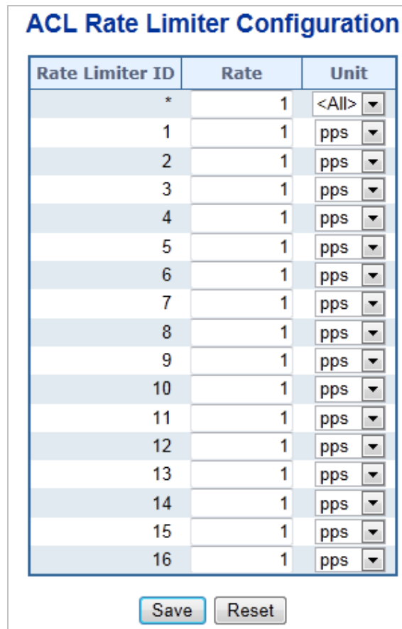
Figure 4-10-5: ACL Rate Limiter Configuration Page Screenshot
