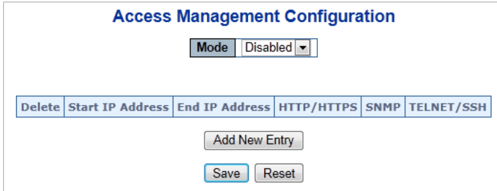
Figure 4-12-2: Access Management Configuration Overview Page Screenshot
