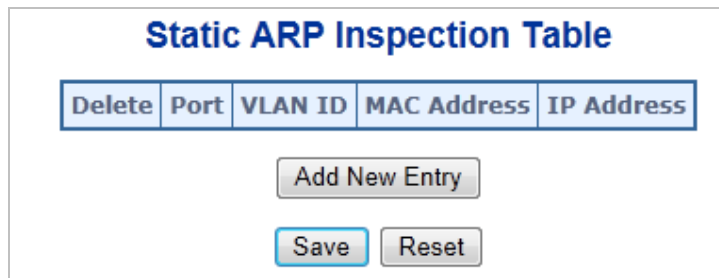
Figure 4-12-13: Static ARP Inspection Table Screen Page Screenshot
