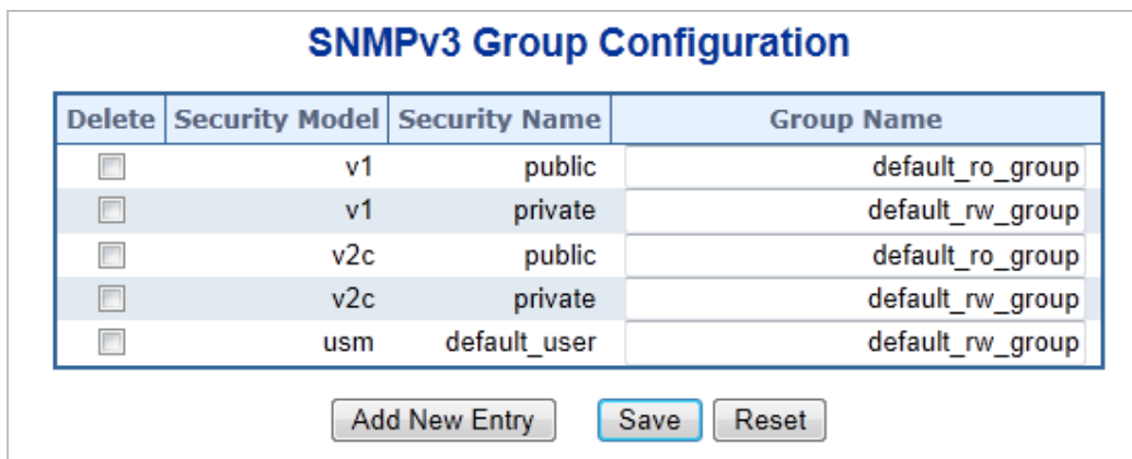
Figure 4-3-5: SNMPv3 Groups Configuration Page Screenshot
