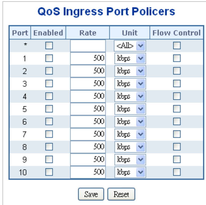
Figure 4-9-1: QoS Ingress Port Policers Page Screenshot
