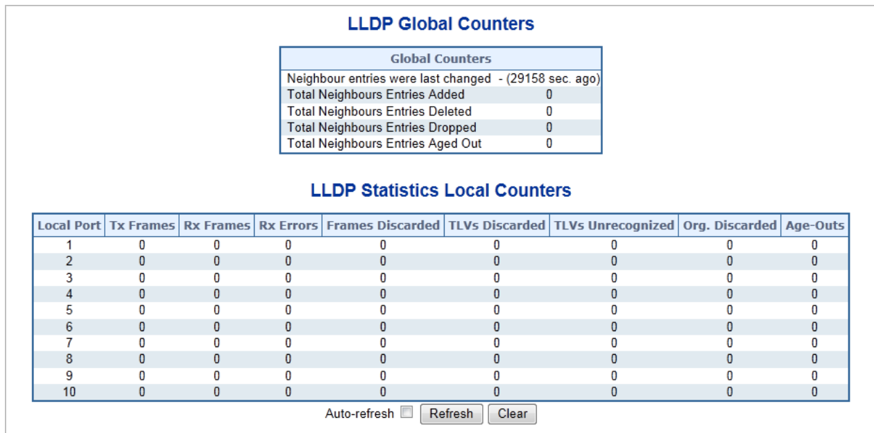
Figure 4-14-5: LLDP Statistics Page Screenshot
