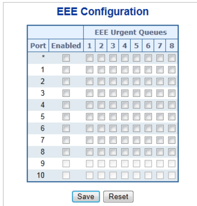
Figure 4-2-21: EEE Configuration Page Screenshot
