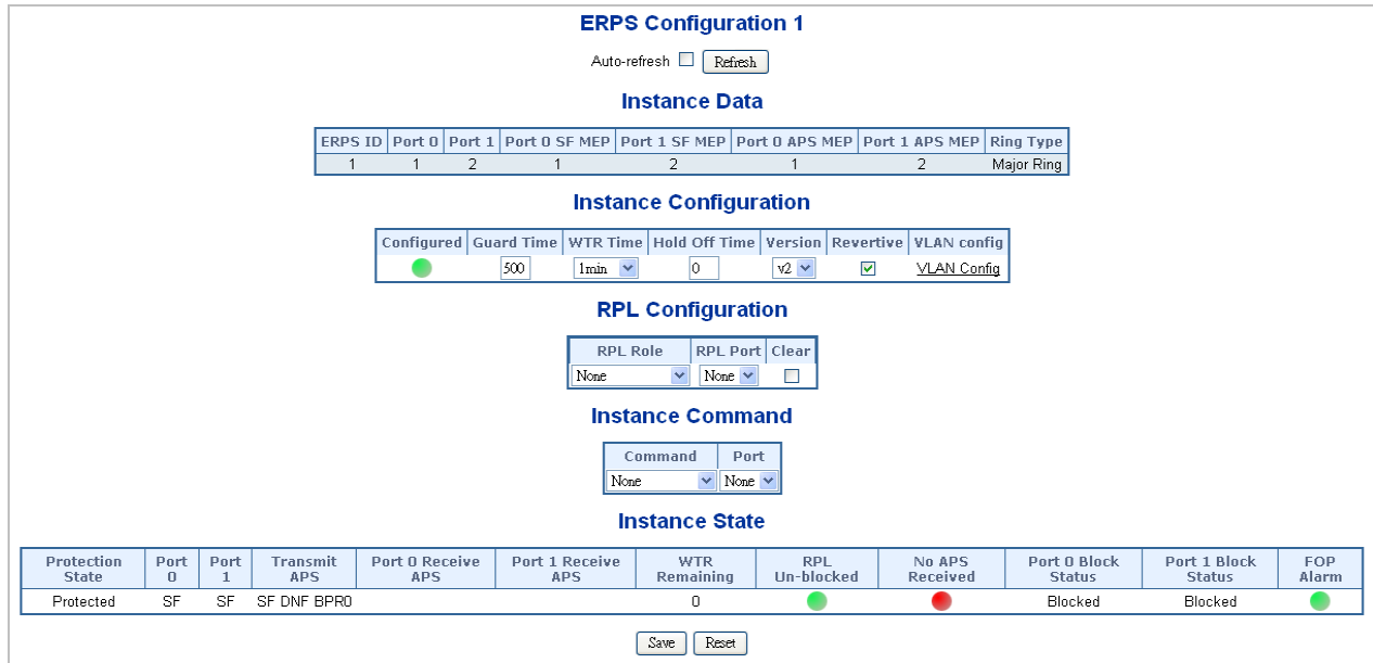
Figure 4-19-4: Ethernet Ring Protocol Switch Configuration page screenshot
