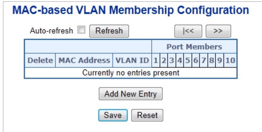
Figure 4-6-17: MAC-based VLAN Membership Configuration Page Screenshot
