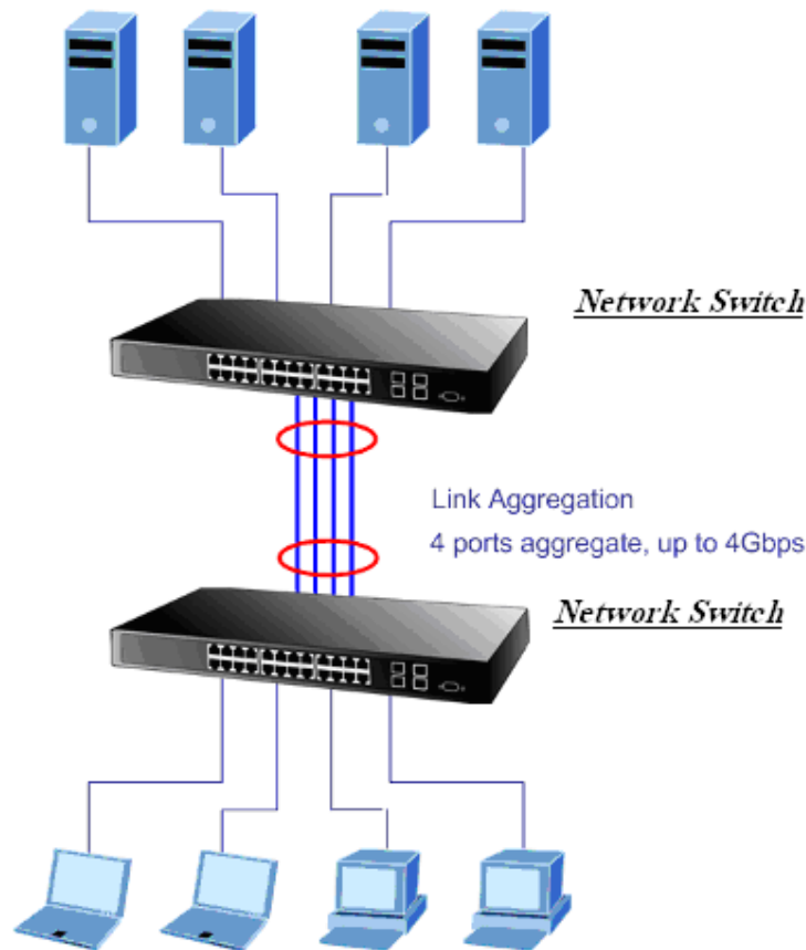
Figure 4-5-1: Link Aggregation Topology
