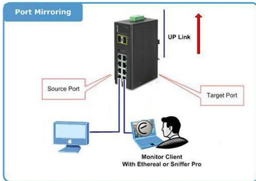
Figure 4-4-5: Port Mirror Application
