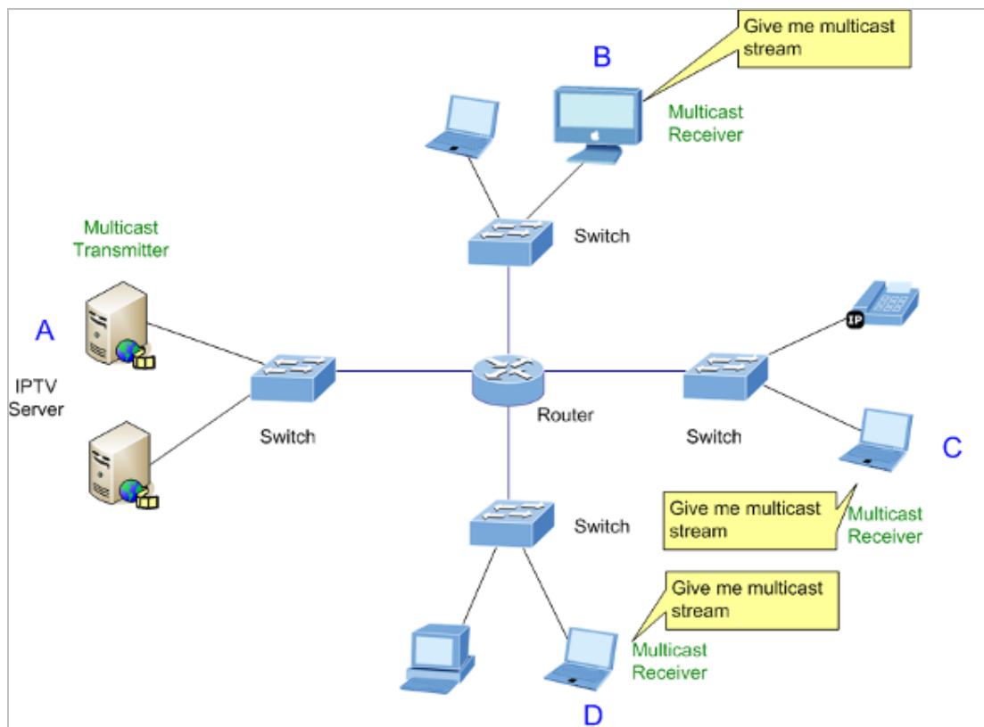
Figure 4-8-1: Multicast Service
