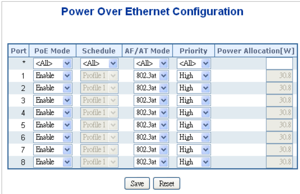
Figure 4-16-3: Power over Ethernet Configuration Screenshot
