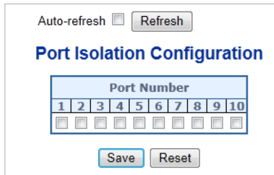
Figure 4-6-7: Port Isolation Configuration Page Screenshot
