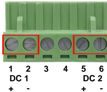
Figure 2-5 6-Pin Terminal Block Power Wiring Input
