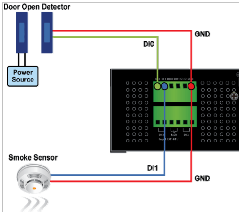
Figure 2-8 Wires DI0 and DI1 to Open Detector
