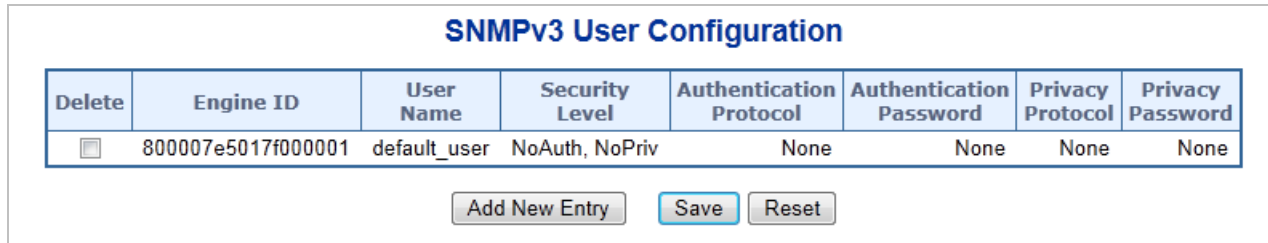
Figure 4-3-4: SNMPv3 Users Configuration Page Screenshot
