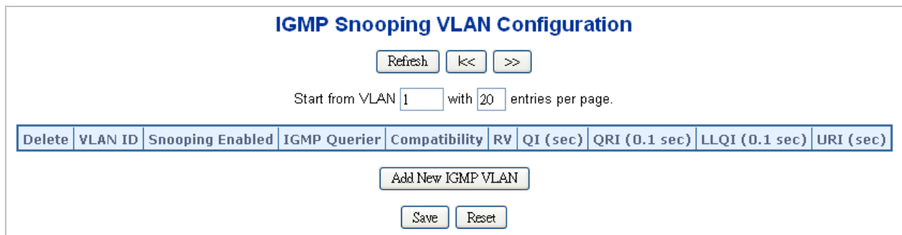
Figure 4-8-6: IGMP Snooping VLAN Configuration Page Screenshot
