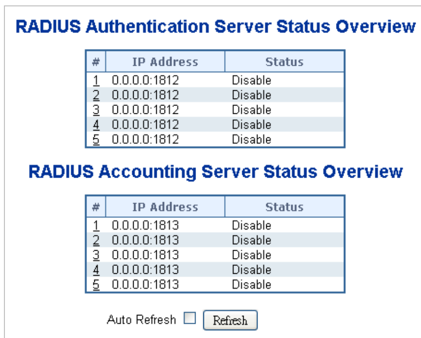
Figure 4-11-8: RADIUS Authentication/Accounting Server Overview Page Screenshot
