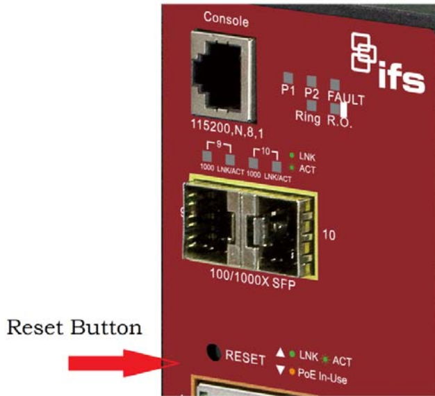
Figure 2-3: Reset button of Industrial Managed Switch
