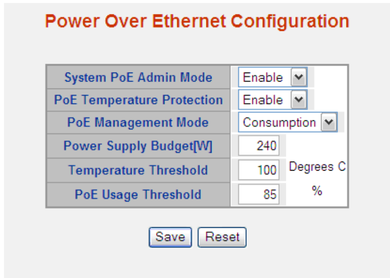
Figure 4-16-2: PoE Configuration Screenshot
