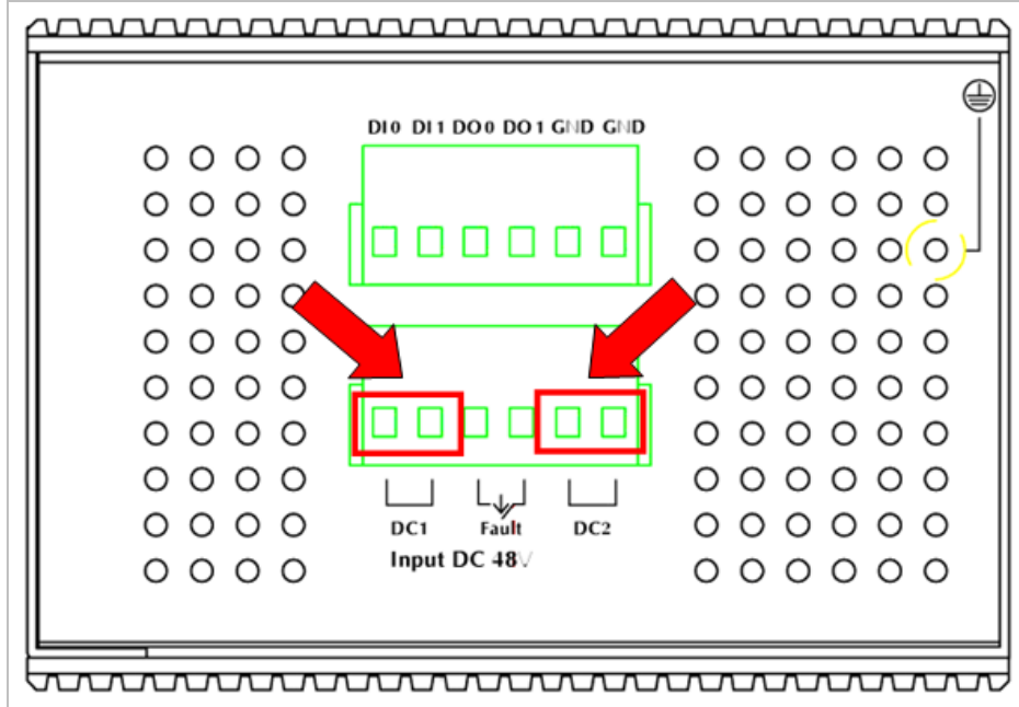
Figure 2-4: NS3552-8P-2S Upper Panel
