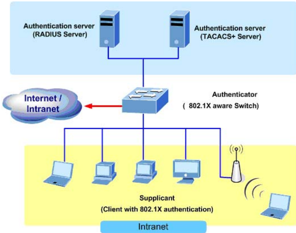
Figure 4-11-1
