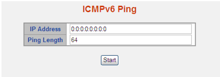
Figure 4-15-2: ICMPv6 Ping Page Screenshot
