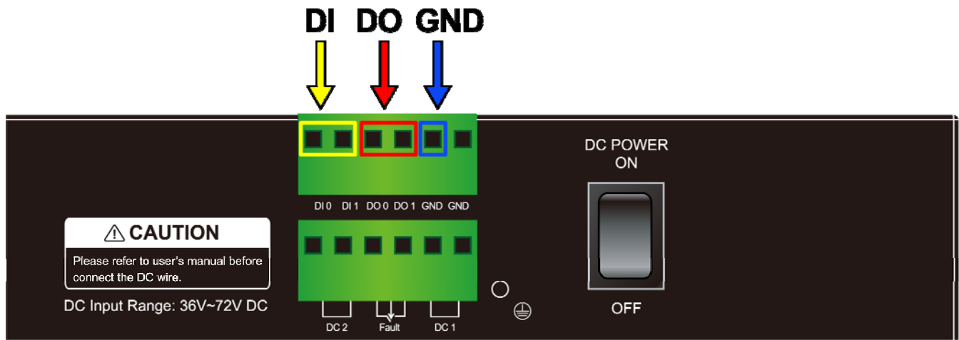
Figure 2-11 Wiring the Redundant Power Inputs
