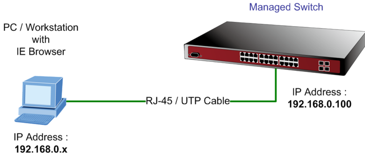
Figure 3-3 Web Management Diagram
