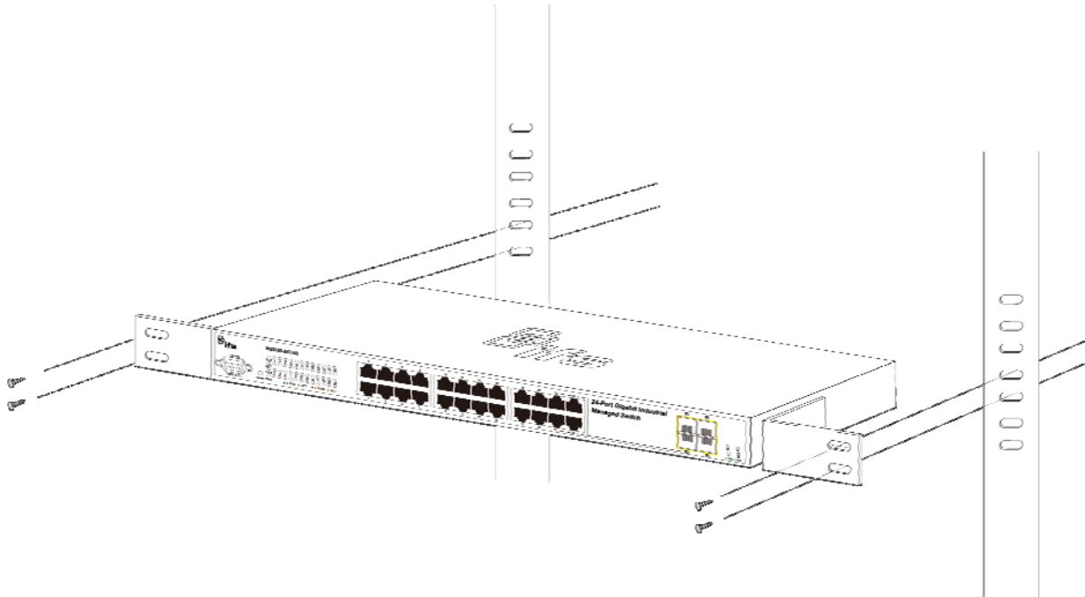
Figure 2-6 Mounting the Managed Switch on a Rack
