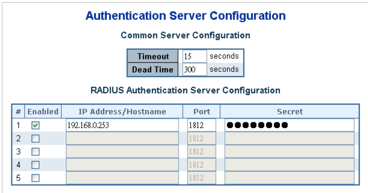
Figure 4-11-10 RADIUS Server Configuration Page Screenshot
