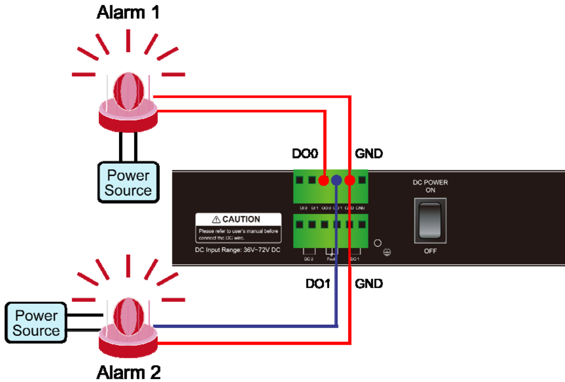
Figure 2-14 Wiring DO0 and DO1 to Open Detector
