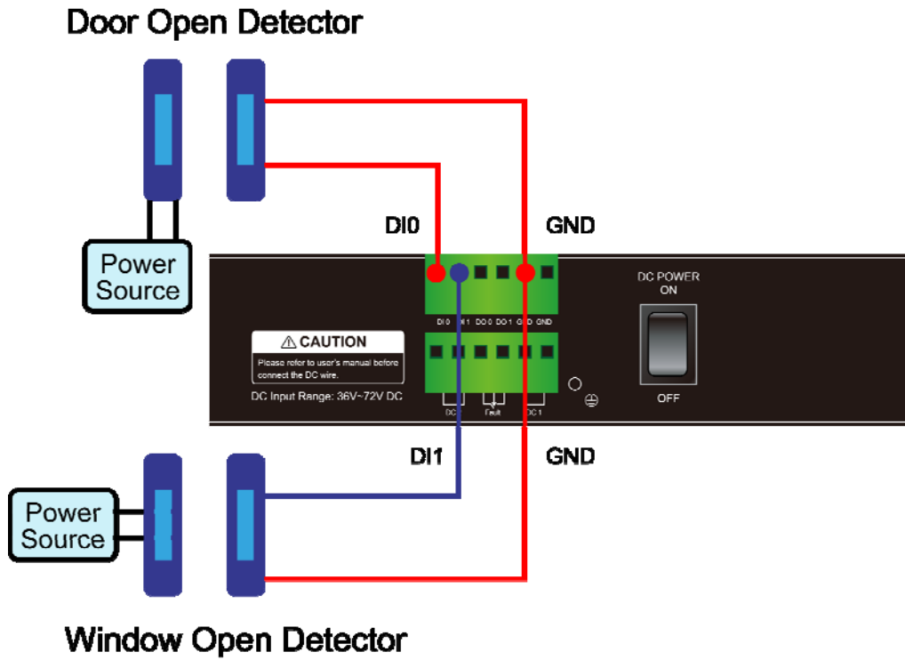
Figure 2-13 Wires DI0 and DI1 to Open Detector
