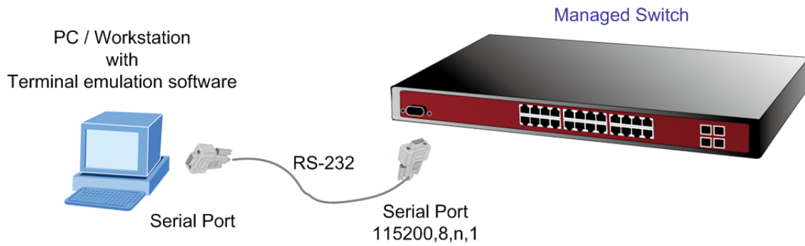
Figure 3-1 Console Management Diagram
