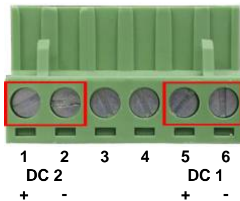
Figure 2-10 6-Pin Terminal Block Power Wiring Input
