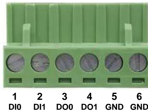
Figure 2-12 6-Pin Terminal Block DI / DO Wiring Input
