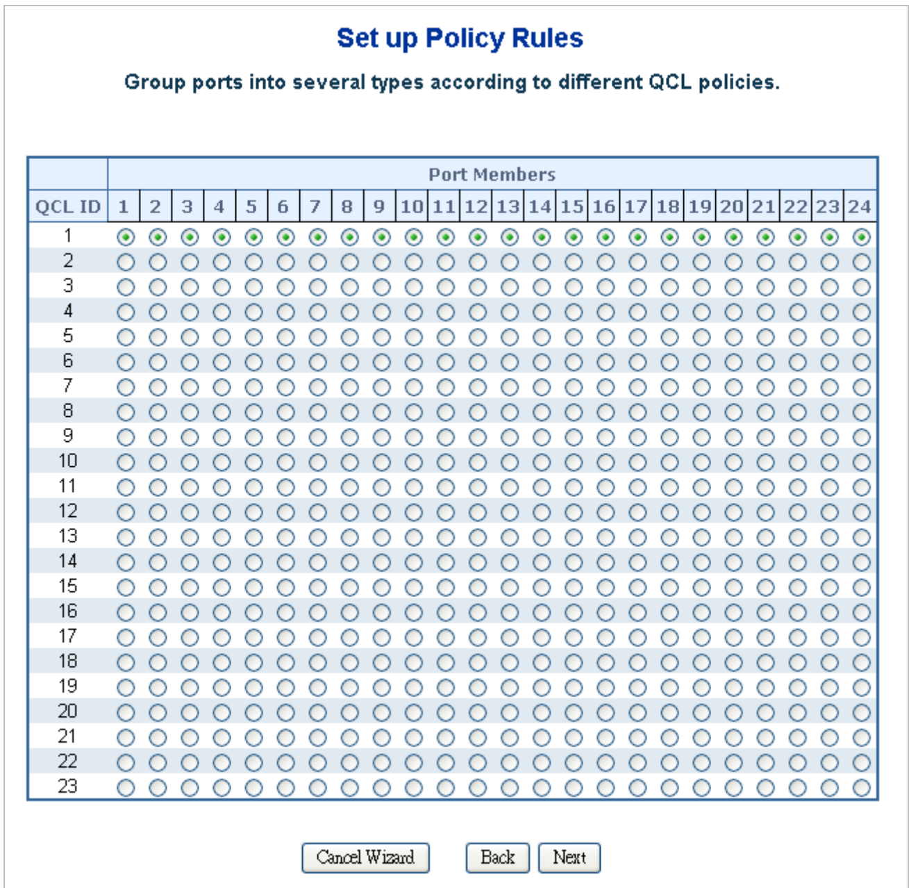
Figure 4-9-2 Set up Policy Rules Page Screenshot
