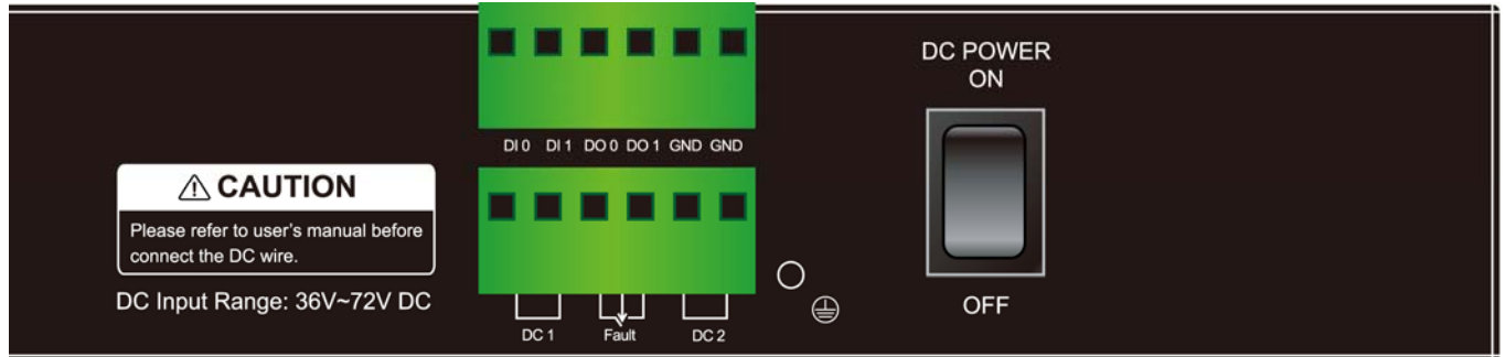
Figure 2-9 Wiring the Redundant Power Inputs
