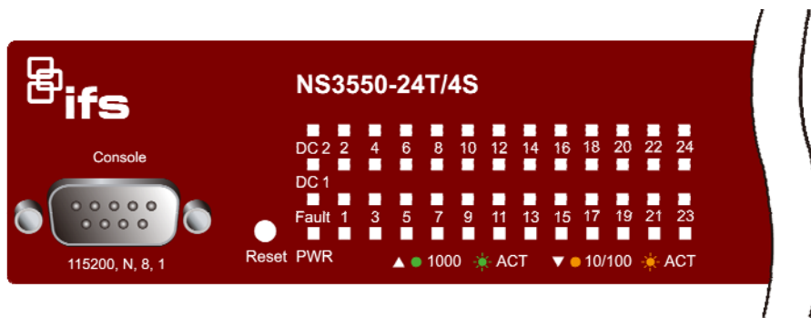
Figure 2-2 NS3550-24T/4S LED Panel
