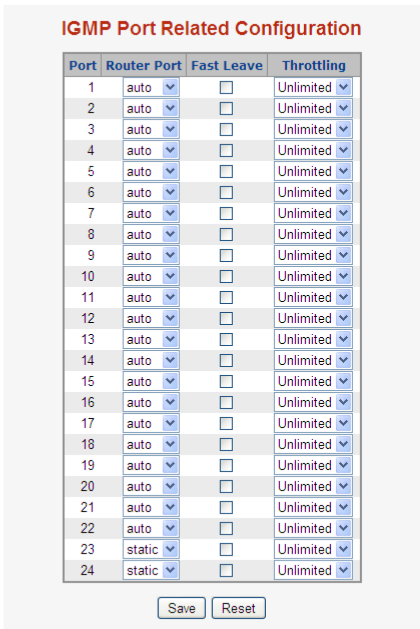
Figure 4-8-6 IGMP Port Related Configuration Page Screenshot
