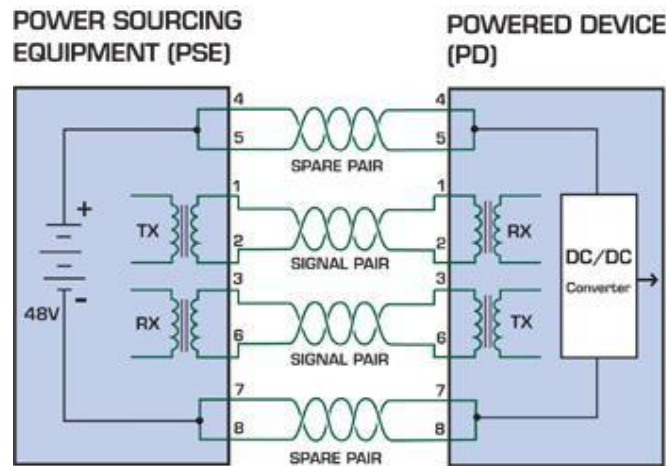
Figure 8-1 - Power Supplied over the Spare Pins
