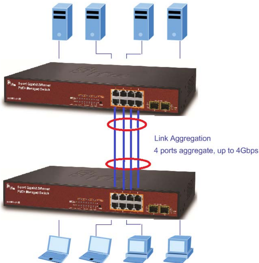
Figure 4-5-1: Link Aggregation
