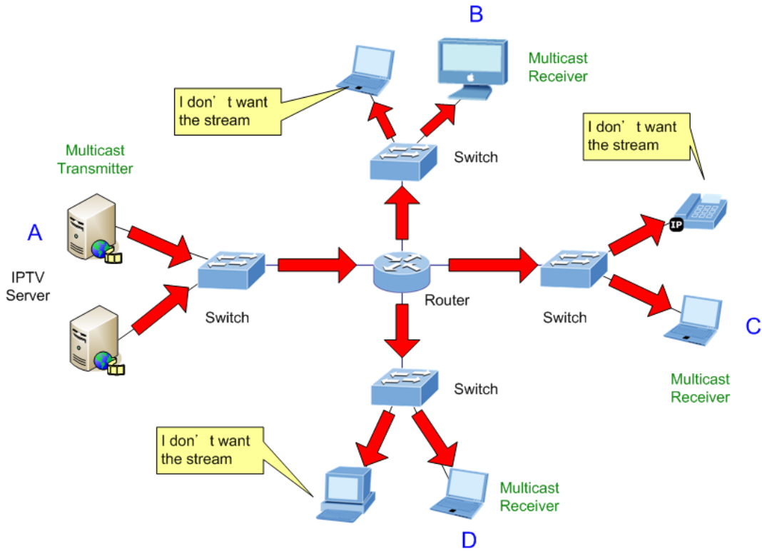
Figure 4-8-2: Multicast flooding
