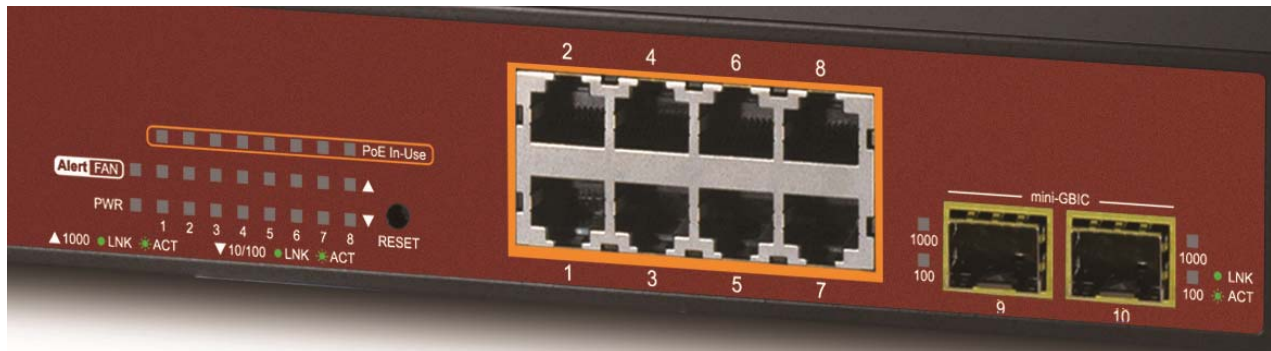
Figure 2-2: NS3502-8P-2S LED panel
