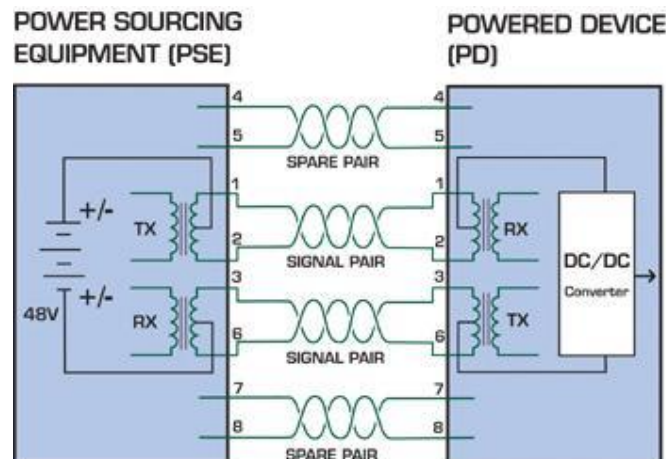
Figure 8-2 - Power Supplied over the Data Pins
