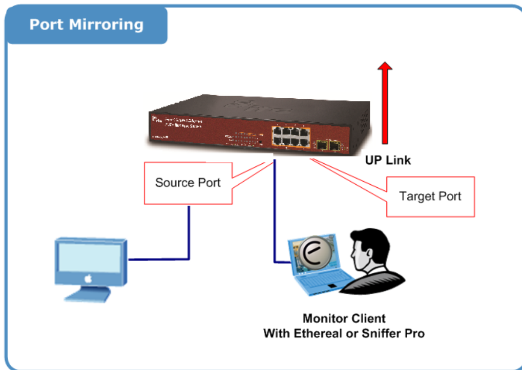
Figure 4-4-6: Port Mirror application
