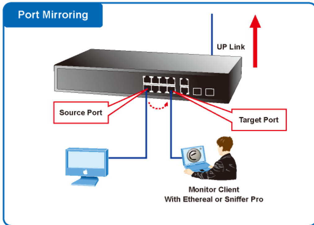
Figure 4-3-5: Port Mirror application
