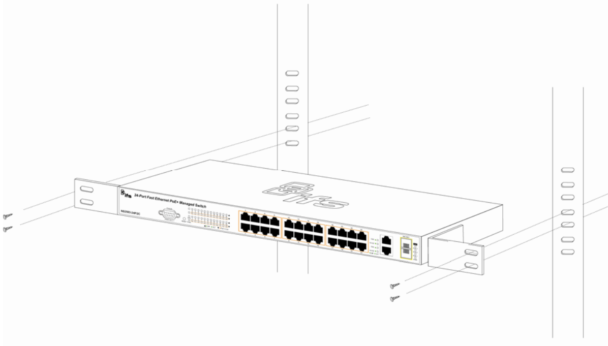
Figure 2-11: Mounting the Switch in a Rack
