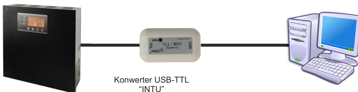
USB-TTL communication using the USB-TTL „INTU” interface.
