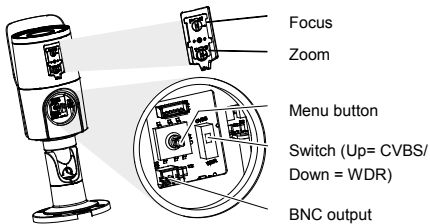
Figure 2: TVB-2404 /TVB-4404
