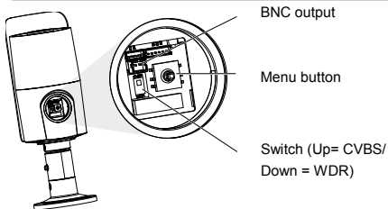
Figure 3: TVB-2405 /TVB-4405
