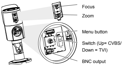
Figure 1: TVB-2402 /TVB-4402
