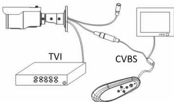
Figure 5: CBSC cable connections
